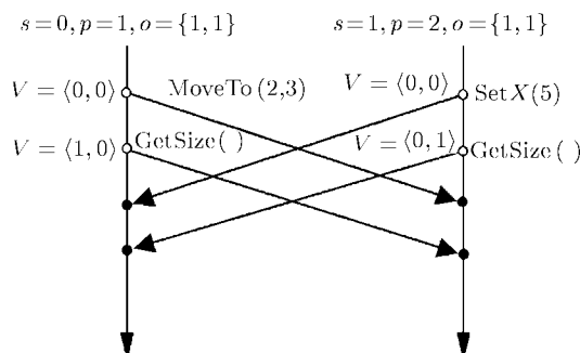
Fig.1. Concurrent operations on an atomic object.
