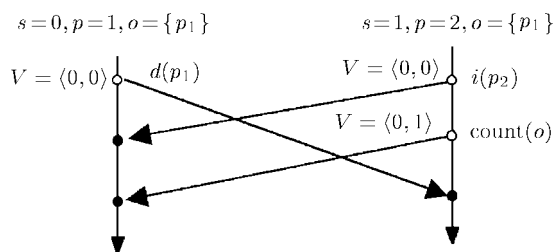
Fig.2. Concurrent operations on a set object.
